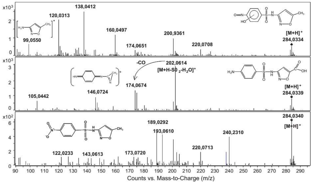
Figure 3. Product ion spectra of three isobaric compounds identified during ozonation processes.
