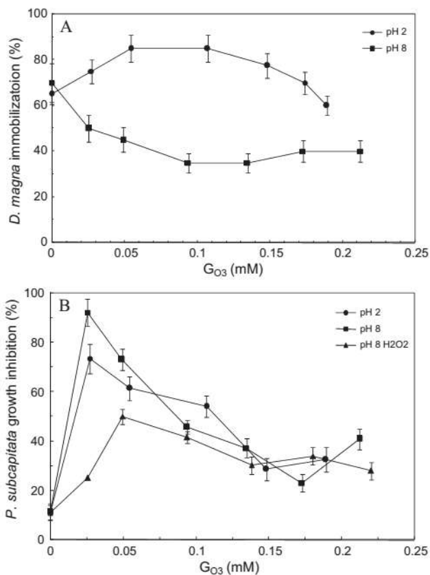
Figure 6. Toxicity assessed by immobilization of D. magna (A, 48 h) and growth inhibition of P. subcapitata (B, 72 h) as a function of the amount of ozone transferred to the liquid phase for runs pH 2 (●), pH 8 (■) and pH 8/H 2 O 2 (▲).
