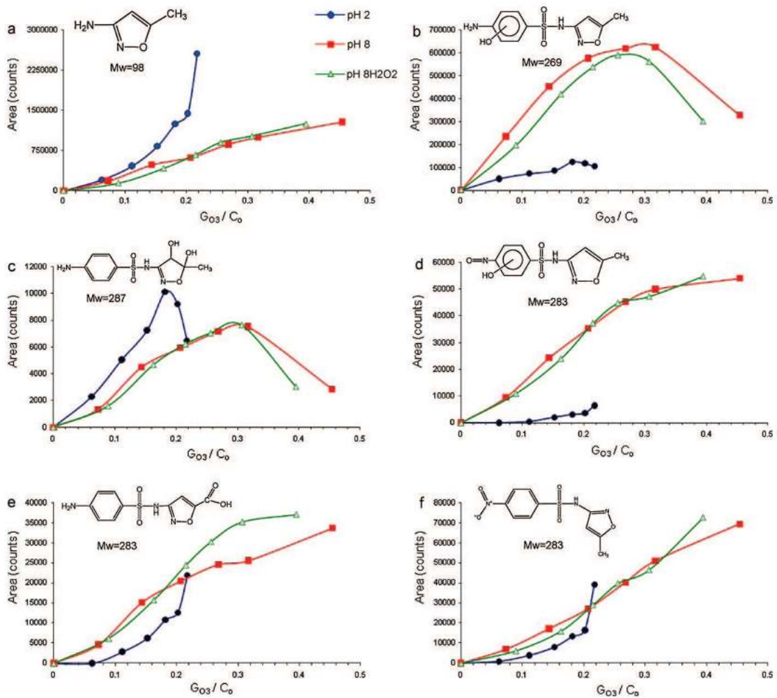
Figure 4. Formation kinetics of the TPs identified during ozonation at pH 2 (●), pH 8 (■) and pH 8/H 2 O 2 (▲).
