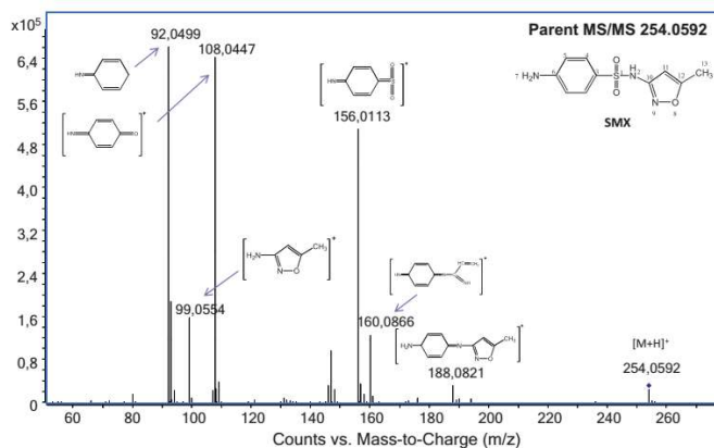
Figure 2. Product ion spectrum of SMX obtained by QqTOF-MS/MS and proposed fragmentation pathway.
