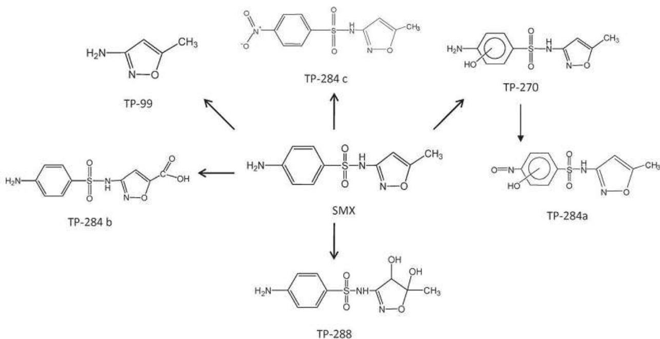
Figure 5. Degradation pathways of SMX, which include: (1) hydroxylation of the benzene ring; (2) oxidation of the amine group at the benzene ring; (3) oxidation of the methyl group at the isoxazole ring; (4) oxidation of the double bond C=C at the isoxazole ring; and (5) S–N bond cleavage.
