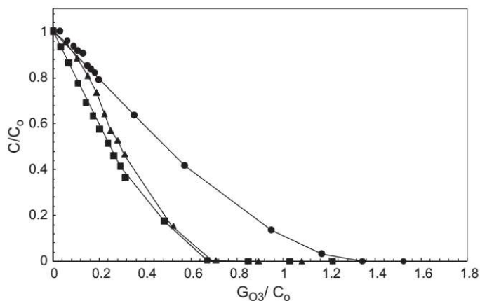
Figure 1. Variation of dimensionless SMX concentration ( C/C_0 ) as a function of the amount of ozone transferred to the liquid per mole initial SMX, G_{O_3}/C_0 for runs pH 2 (●), pH 8 (■) and pH 8/H 2 O 2 (▲).
